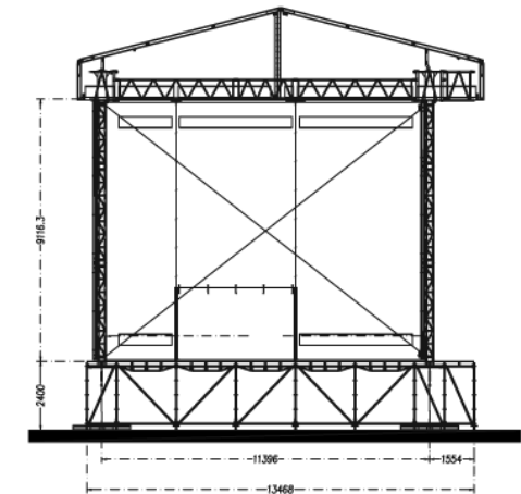
Side view off-stage section.
