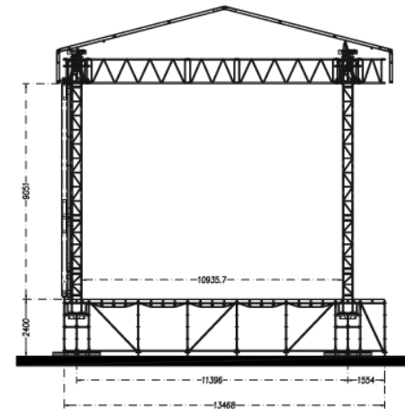
Side view middle section.
